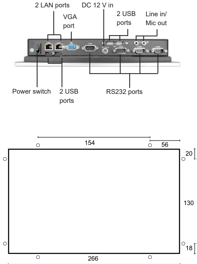
Mounting holes
